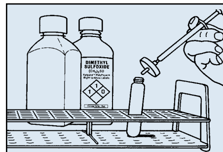
Fig. 3 Sterilization of DMSO by filtration.
